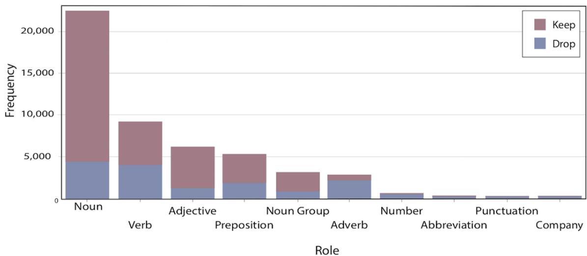
Figure 2. Parts of speech from text filtering: roles by frequency.
