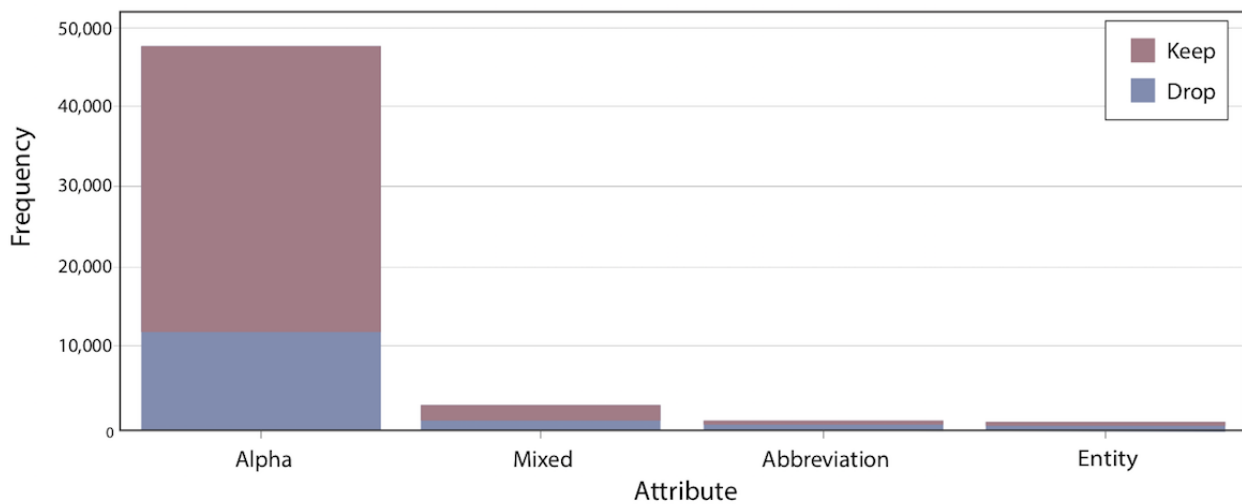
Figure 1. Text filtering results: attributes by frequency.
